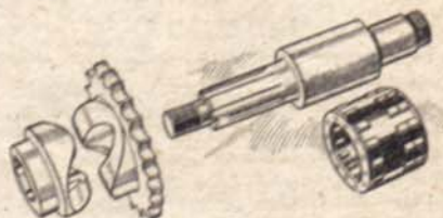
The mainshaft of the "D"-type engine has been increased in diameter and now runs in three rows of caged rollers, while splines for the shock-absorber are formed on the end of the shaft
