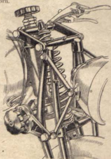
As a result of modifications the front forks fitted to machines in the "D" series now have a greater range of movement. Note the round-section tubing of which the fork girders are built, the heavier links and the rear-positioned shock-dampers
