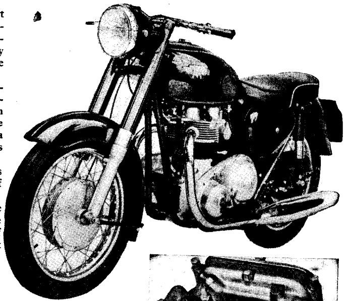
Above: The handsome 646 cc Matchless Majestic. Right: On the Matchless scrambler engine the central plug position shortens flame travel and so permits a high compression ratio
