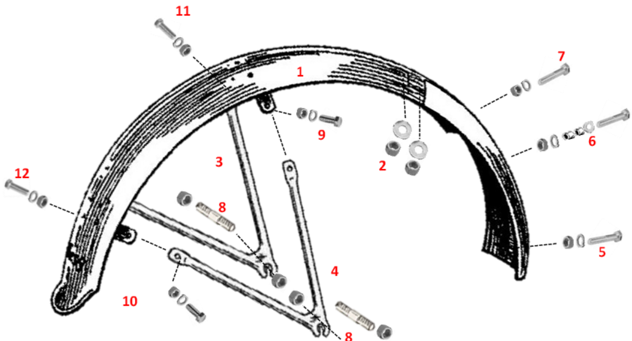
Figure 2: No rib in the centre of mudguard. Removable rear section joint for the mudguard is under the rear of the saddle.
