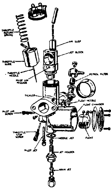
The new Monobloc carburetor features a float bowl and mixing chamber cast as one unit. A hinged float and nylon float needle are used.
