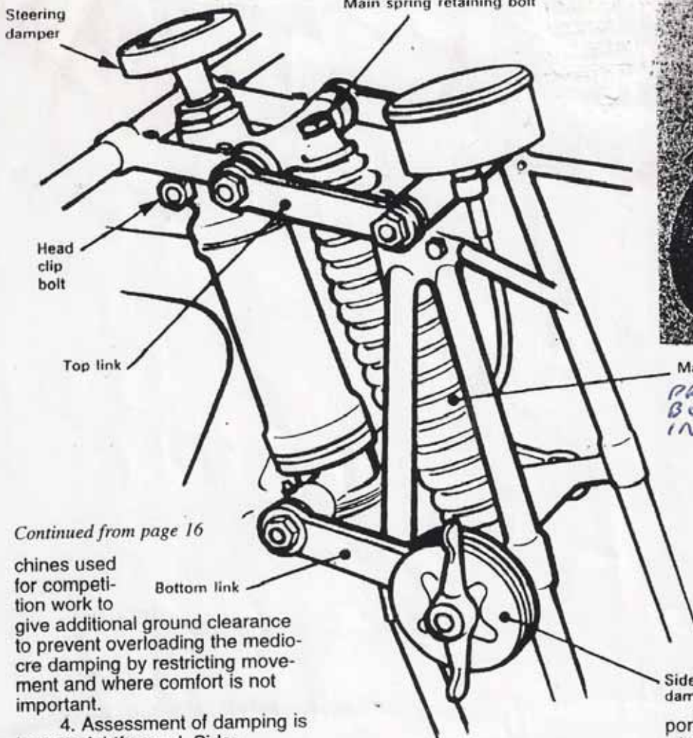
Diagram of a typical Webb-type girder fork.
