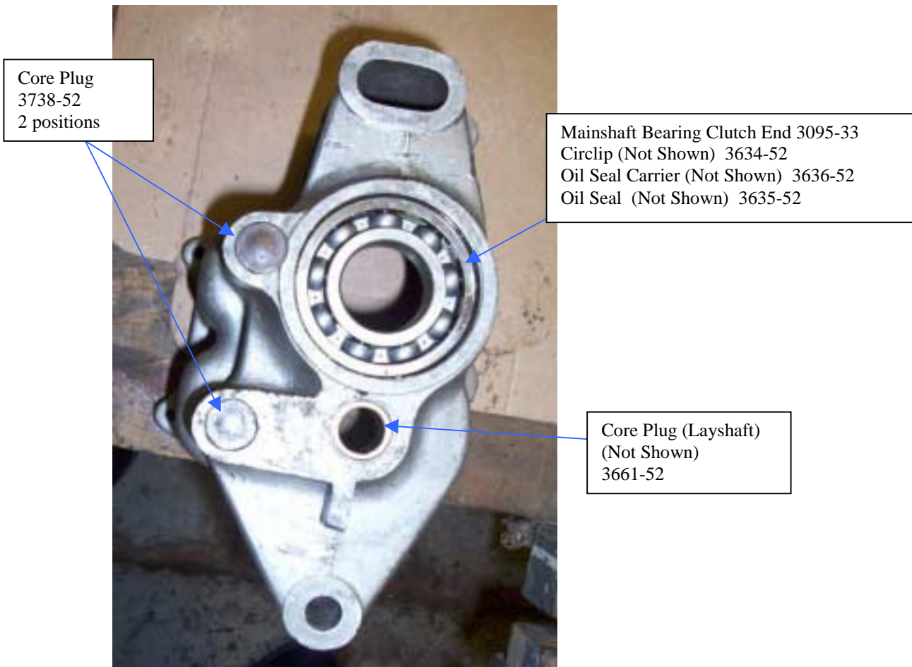
View on Clutch End of Main Case
