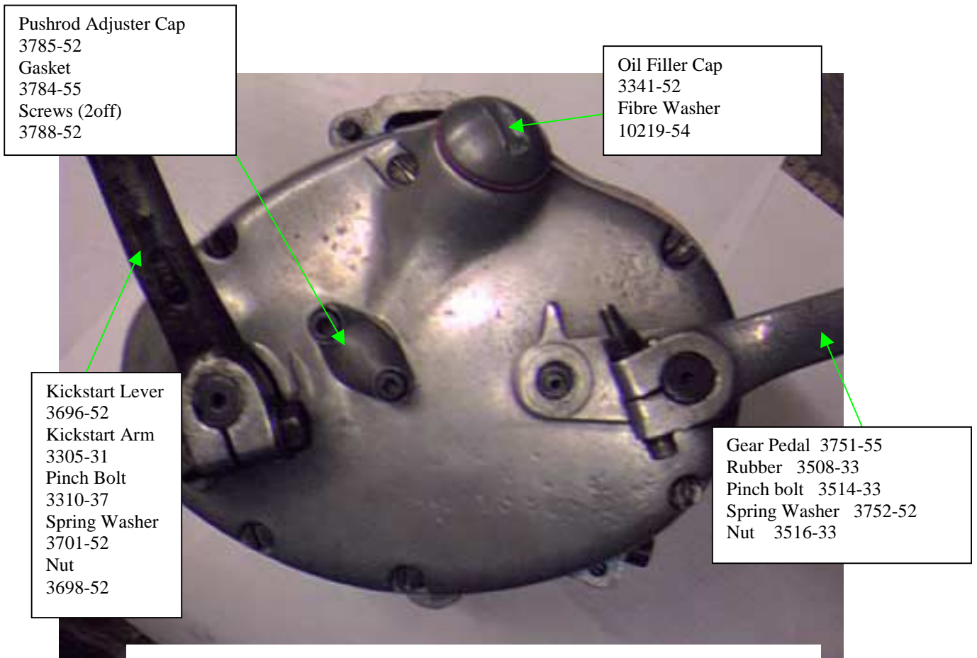
View on Outside of Outer Kickstart Case
