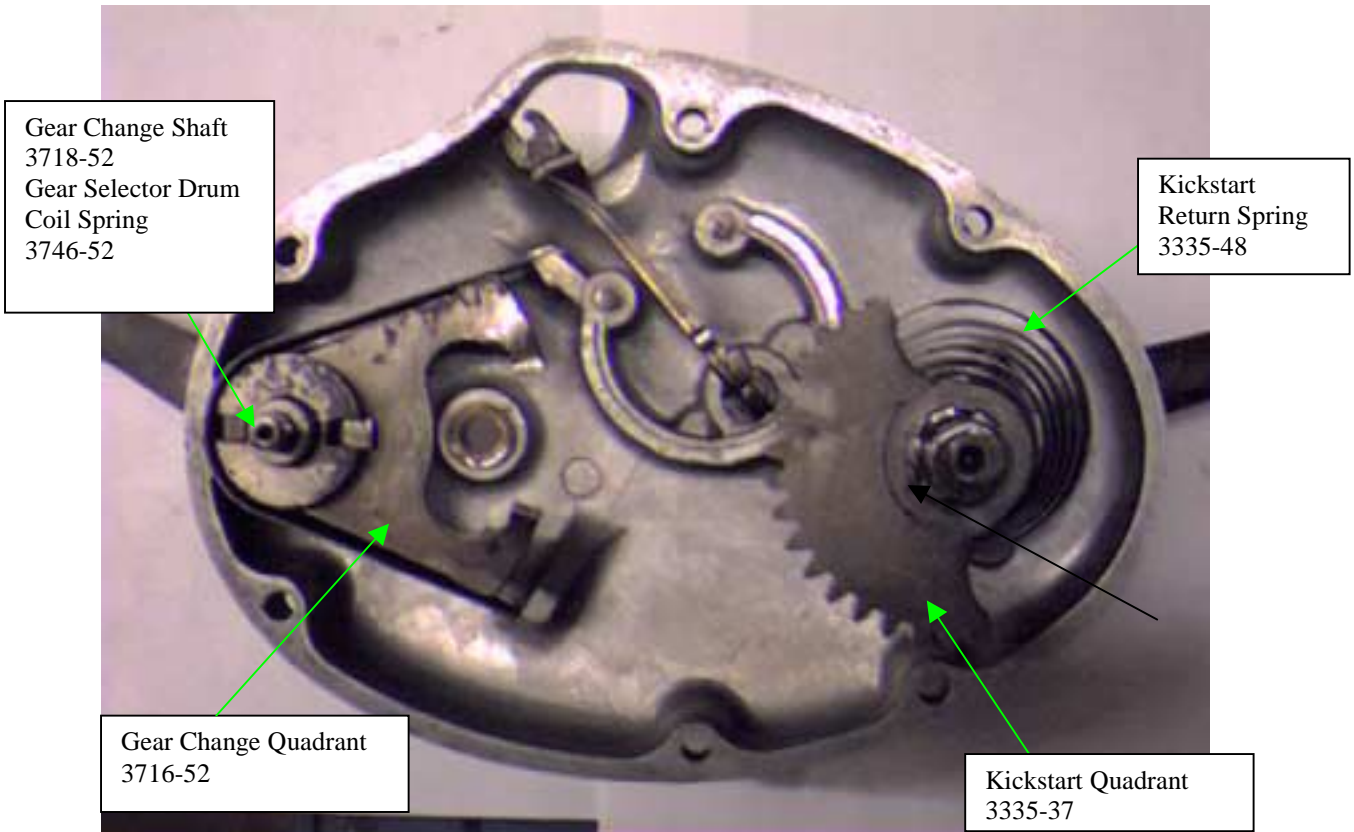
View on Inside of Outer Kickstart Case
