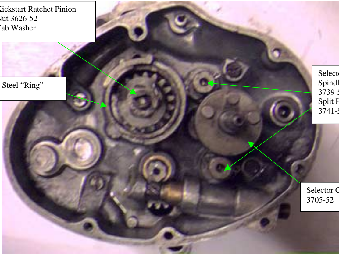
View on Outside of Inner Kickstart Case
