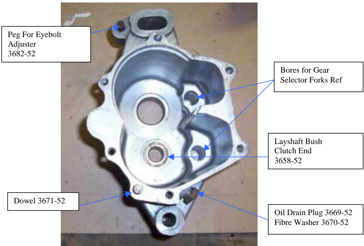
View on Kickstart End of Main Case
