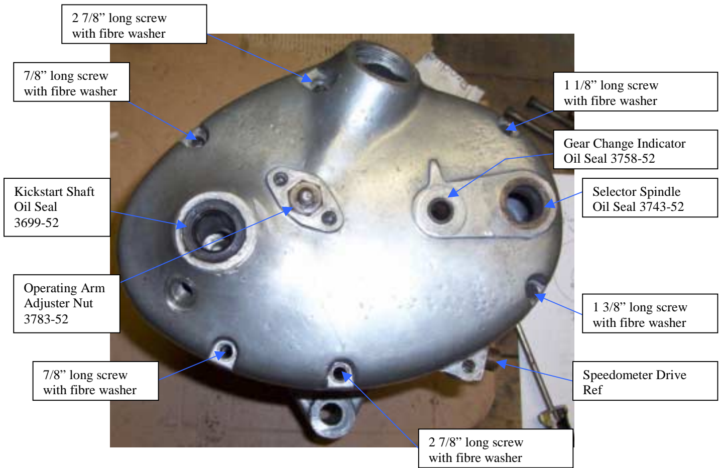
View on Outside of Kickstart Case
