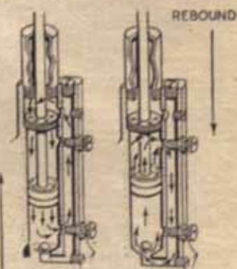
Action of the two-way hydraulic damping shown diagrammatically. Adjustment of the metering screws regulates the damping
