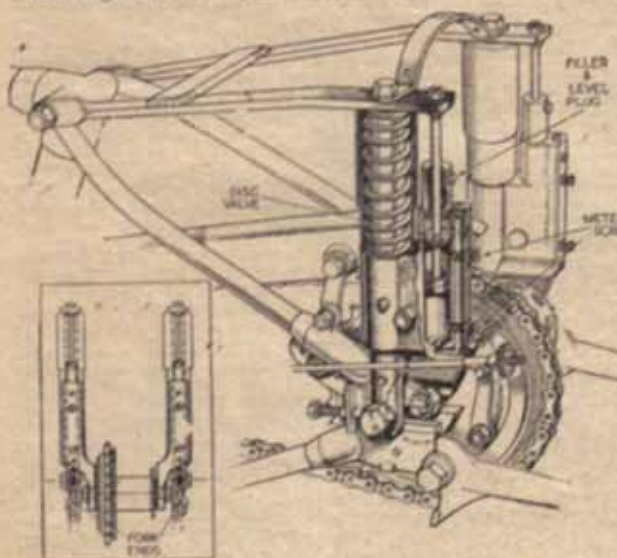
(Above) The wheel spindle is supported by aluminium castings which slide on stout steel bearing posts clamped to the frame. Inset diagram is a rear end elevation
