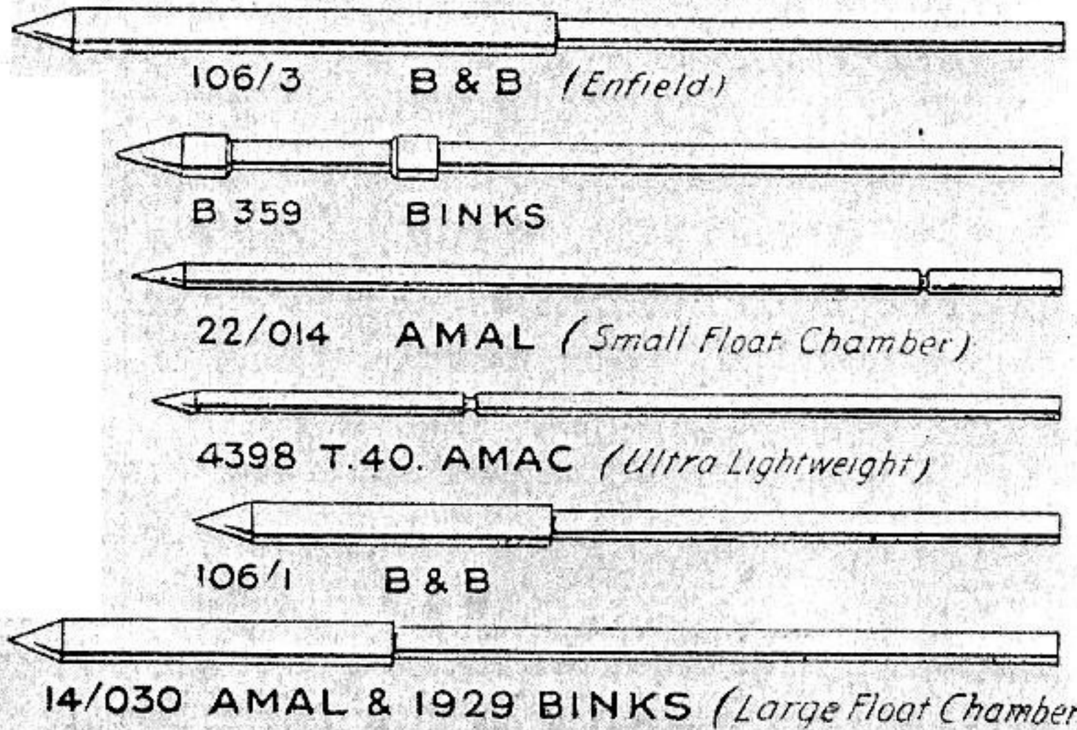
Various "Amal" Float Chamber Needles. Illustrations actual size.
