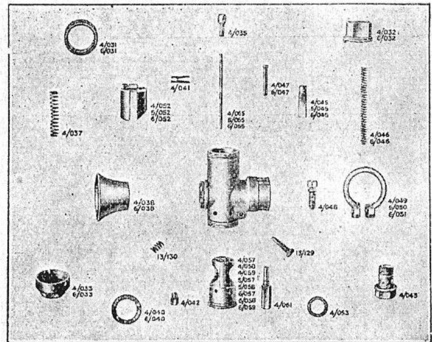
Amal Mixing Chamber Parts
