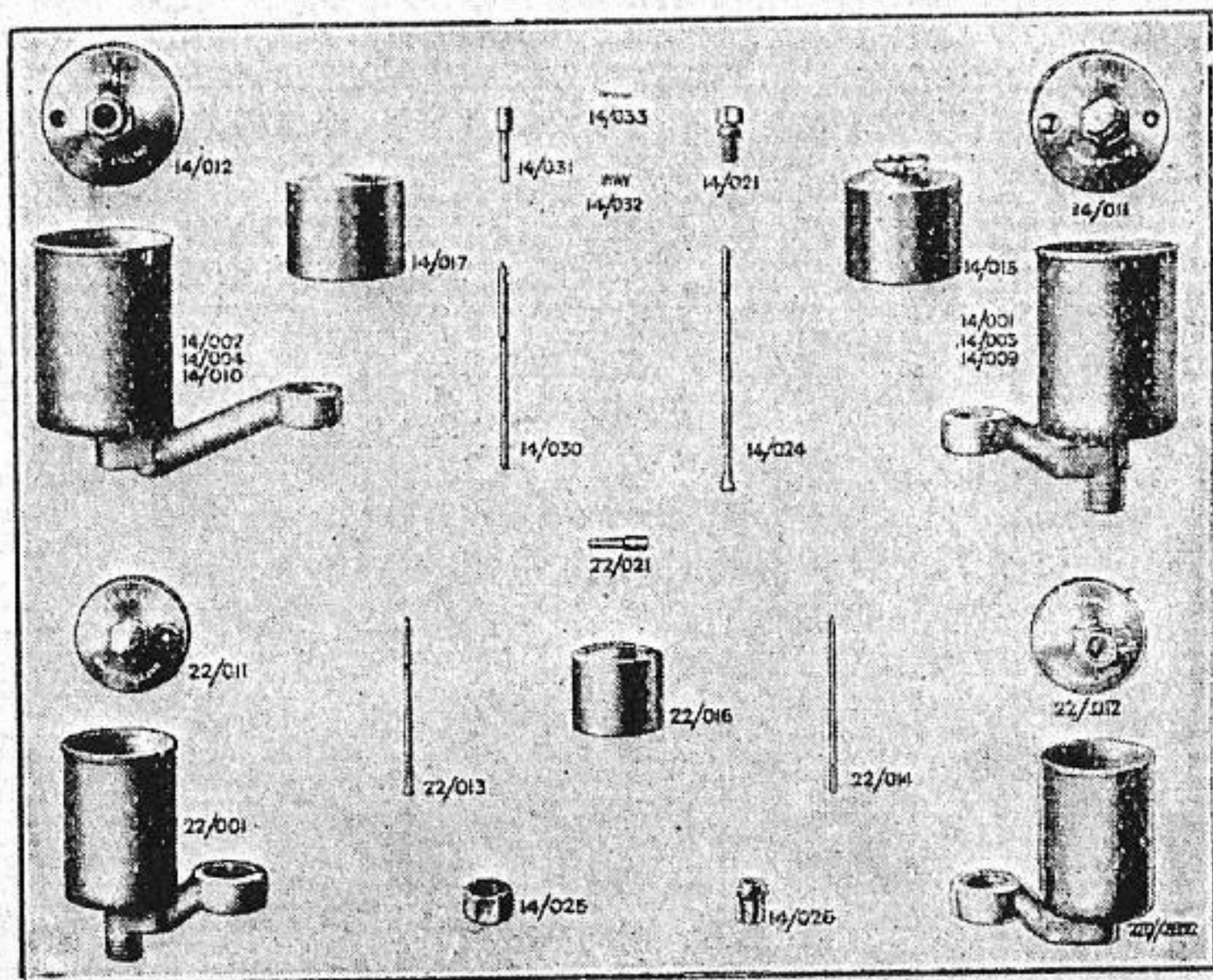
Spare Parts of Float Chambers
