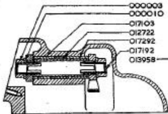
SCRAP SECTION THROUGH ROCKER SHAFT.
