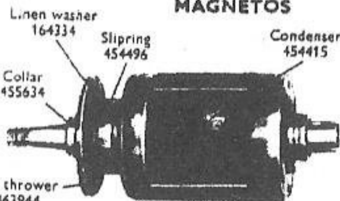
TYPICAL N14 ARMATURE
