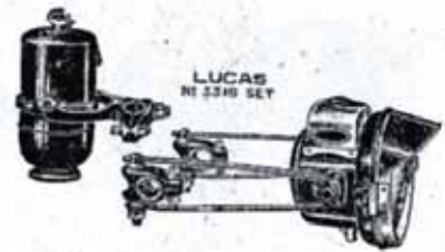
"LUCAS" PROJECTOR SET
